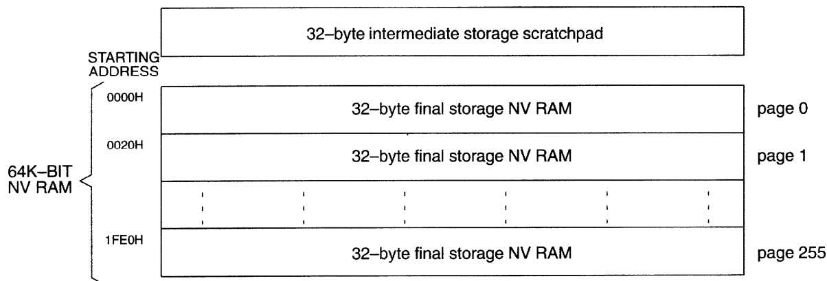
DS1996 MEMORY MAP Figure 5
