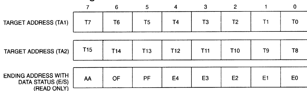
ADDRESS REGISTERS Figure 6
